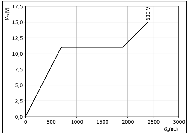
figure 13. IGBT
