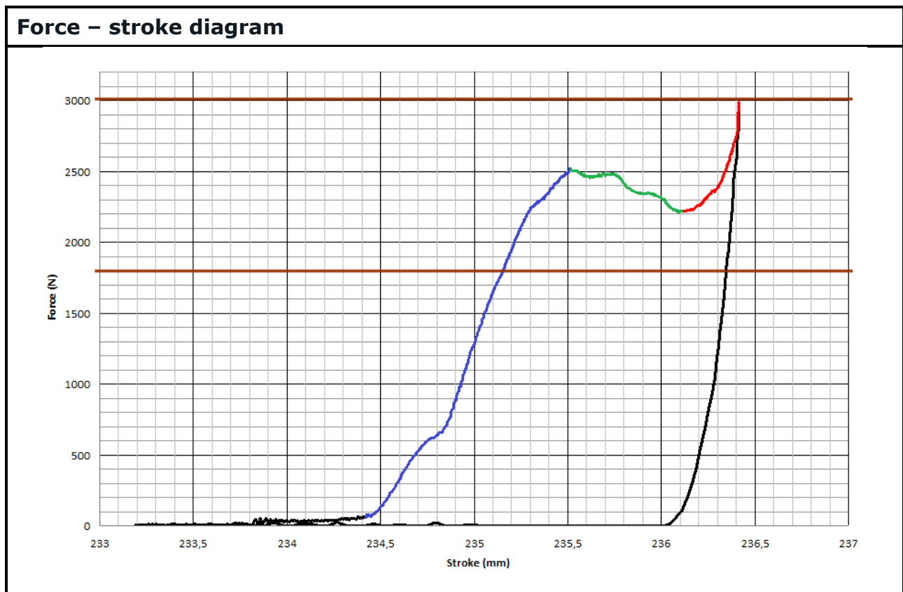
Figure 22: Typical press-in diagram of a 20 pin module
